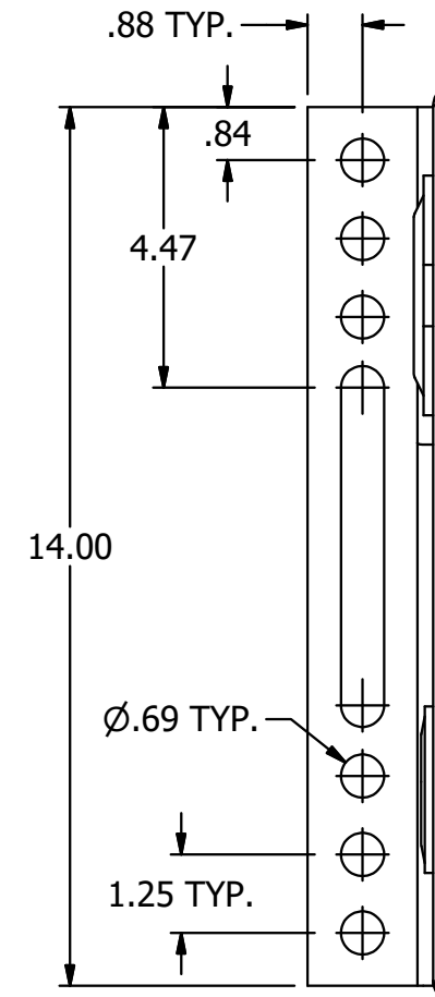
DETAIL A
