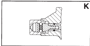
K 2K, 2-Position Detented Cap 3K, 3-Position Detented Cap
