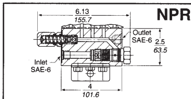
NPR Priority Inlet with Direct Acting Relief Adjustable in 2 Pressure Ranges 50-500/500-3000 psi (3.5-35/35-207 BAR)
