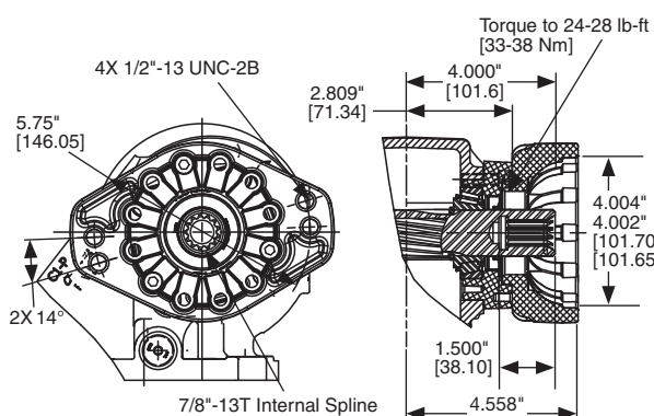
7/8"-13T Internal Spline
