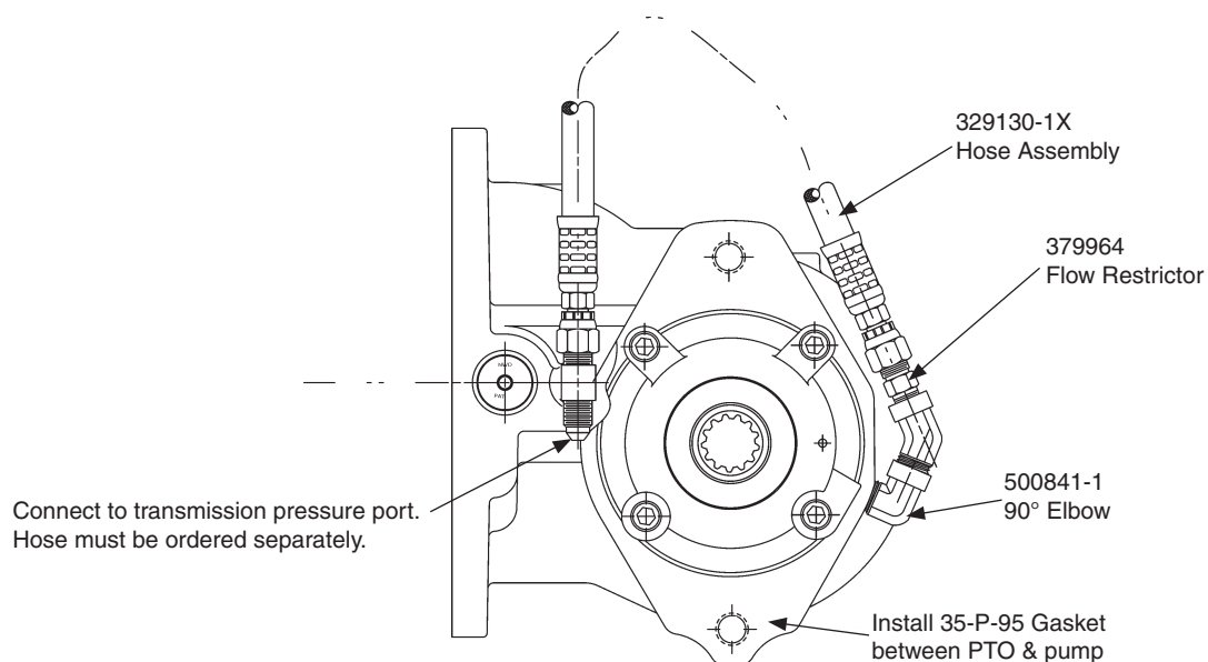
3 ASSY View
