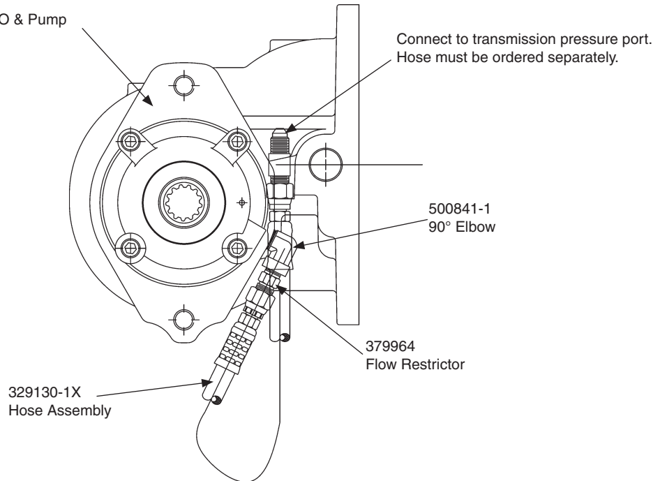
5 ASSY View
