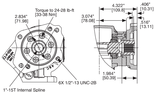
1"-15T Internal Spline
