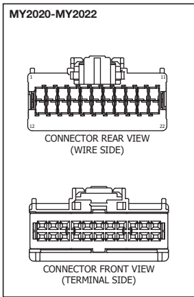
Ford Interface Connector Detail Male Connector (Shown) Provided with Vehicle
