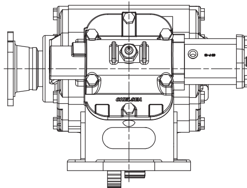
Assembly 6
