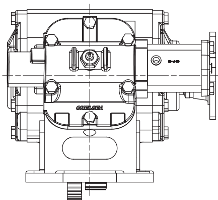
Assembly 3
