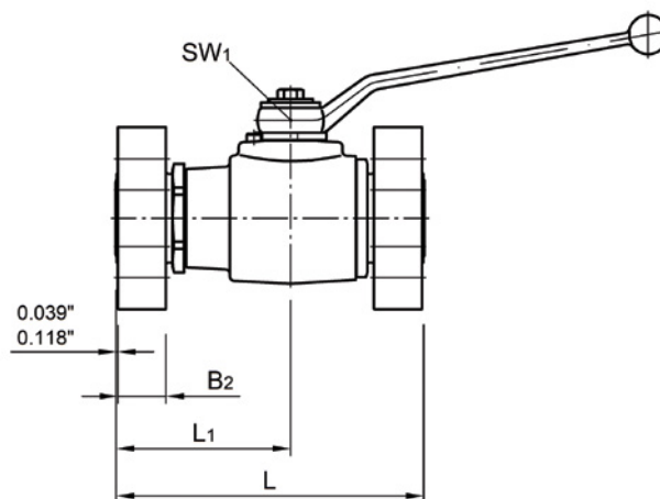
ABF SERIES CODE 61/CODE 62
