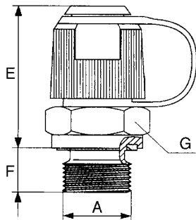
Plastic Cap
