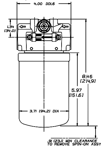
Short Assembly
