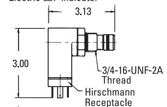
Electric \Delta P indicator with pop-up visual button and manual reset
