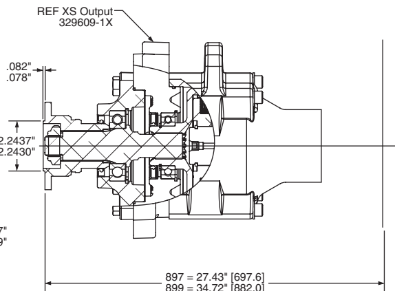
Ass'y "3" & "5"
