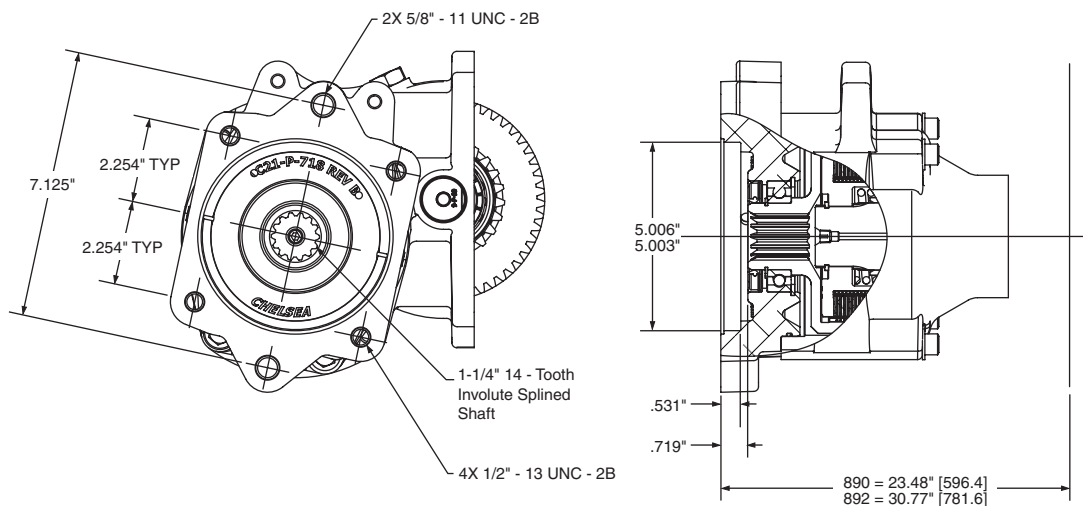
Ass'y "5"
