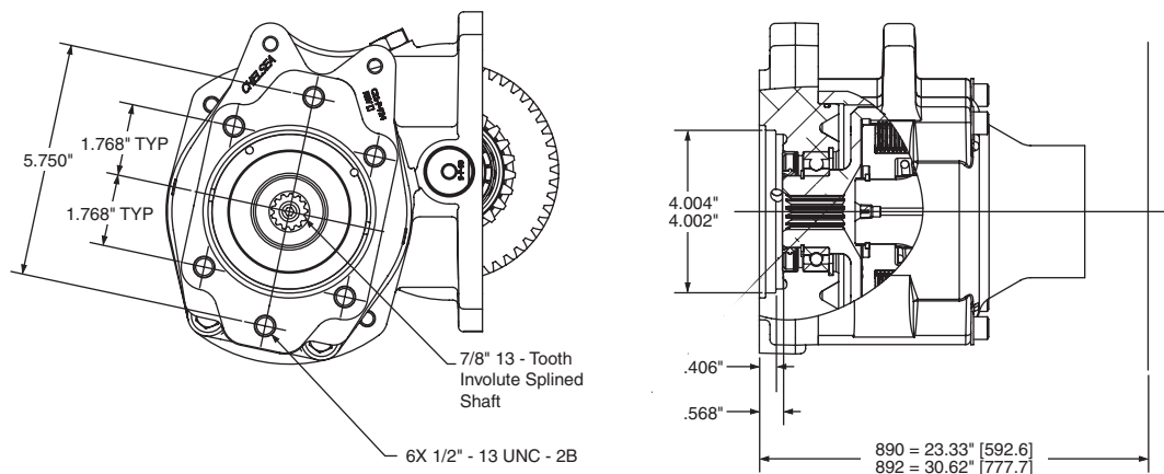
Ass'y "5"
